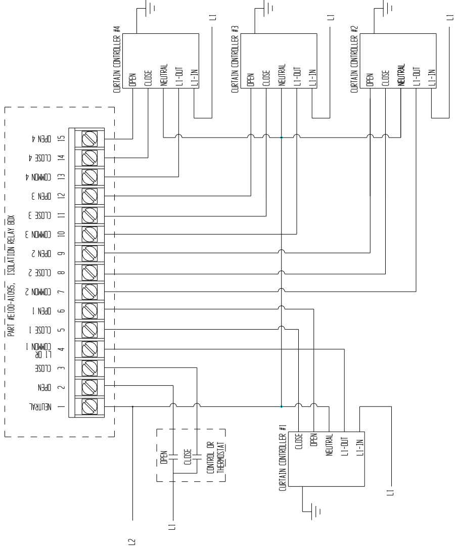
HOO-K-UP DIAGRAM FOR ISOLATING CURTAIN CONTROLLERS
