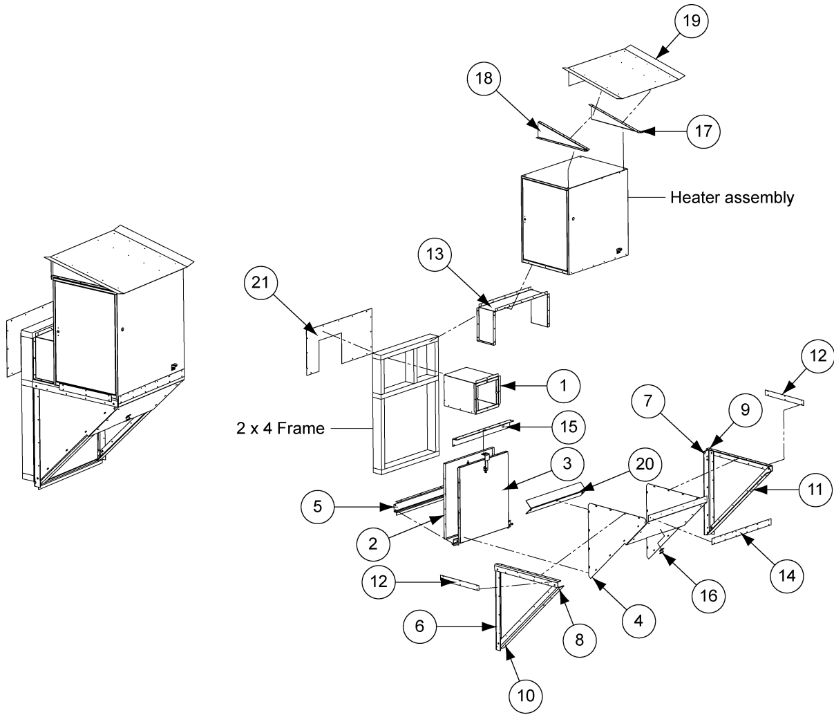
Complete assembly of 41-8000AA
